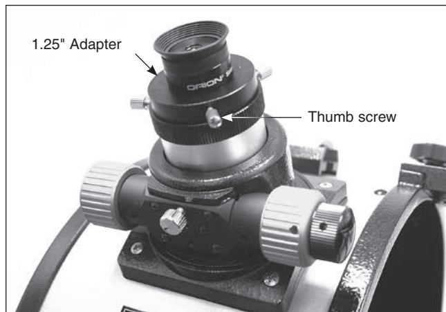
Figure 34. The 1.25" Sirius Plössl eyepiece installed in the focuser's removable 1.25" adapter.
