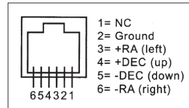
Figure 3b. This is the pin diagram for the SSAG and ST-4 compatible mounts.
