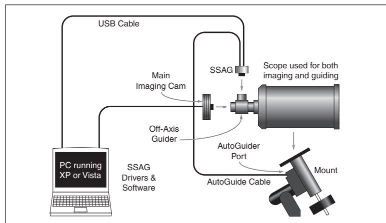
Figure 1b. Cassegrain style telescopes can be used with an off-axis guider. This allows both the main imaging camera and autoguiding to use the same telescope.
