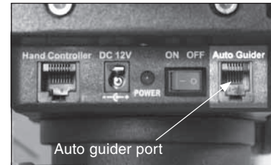
Figure 3a. The SSAG works with any mount equipped with an ST-4 compatible autoguider port, shown here on the Sirius EQ-G mount.
