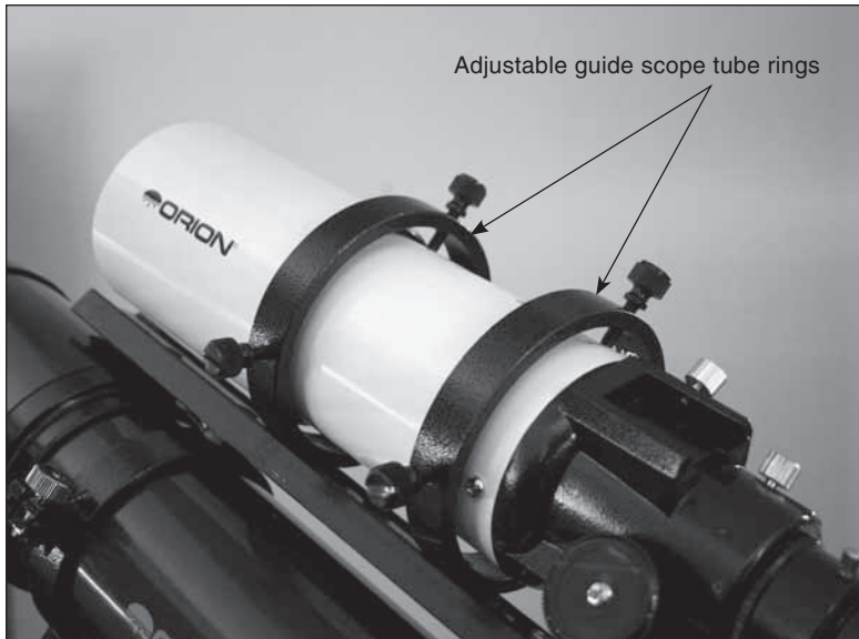
Figure 2. Adjustable guide scope tube rings allow you to adjust the position of the guide scope without moving the main imaging scope.
