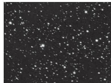
Figure 4. Field Rotation occurs in long exposure images taken with an altitude-azimuth mount or poorly polar aligned equatorial mount.
