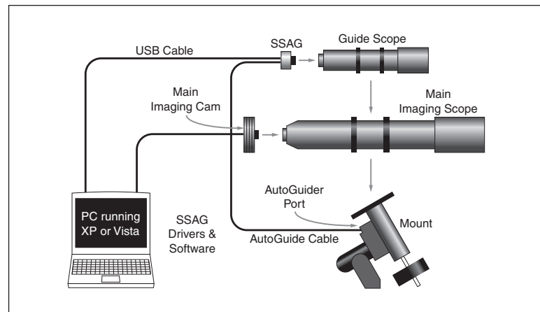
Figure 1a. A traditional imaging setup contains a main imaging scope and separate guide scope. The SSAG interfaces with your computer via the USB cable, and connects to your mount's autoguide port via the autoguide cable.
